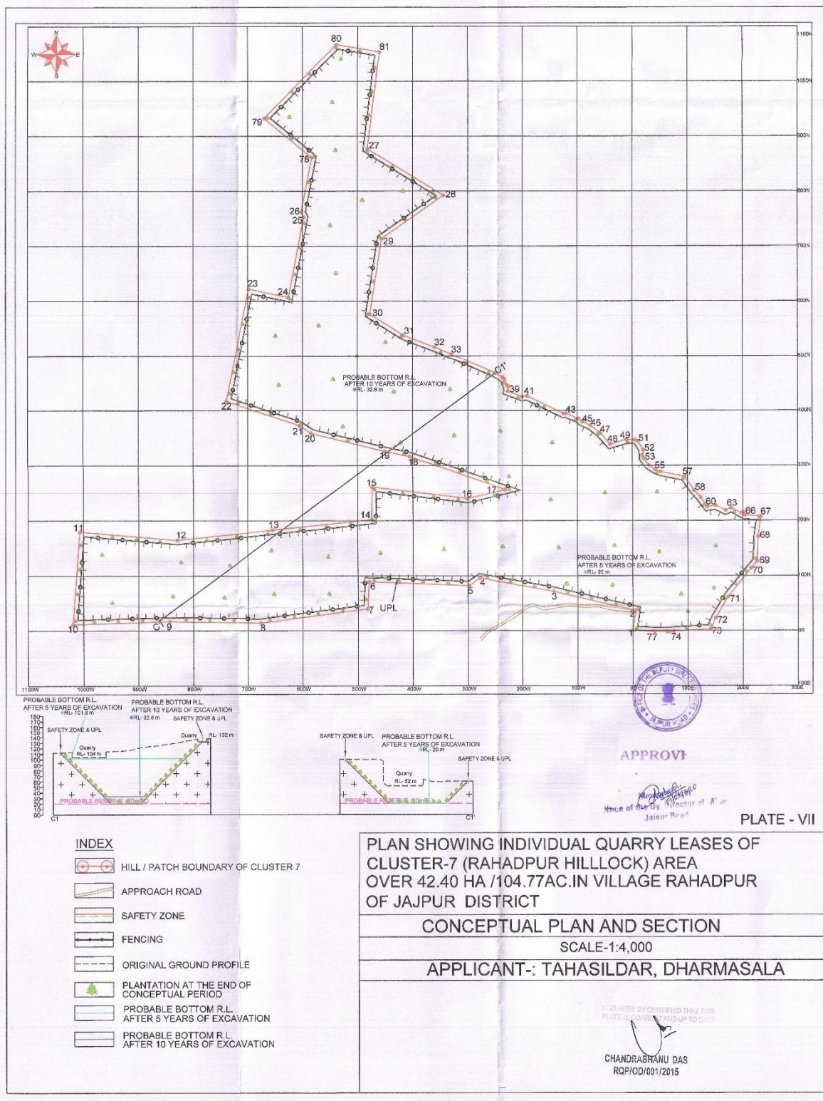
Figure 2.4: Conceptual Plan
