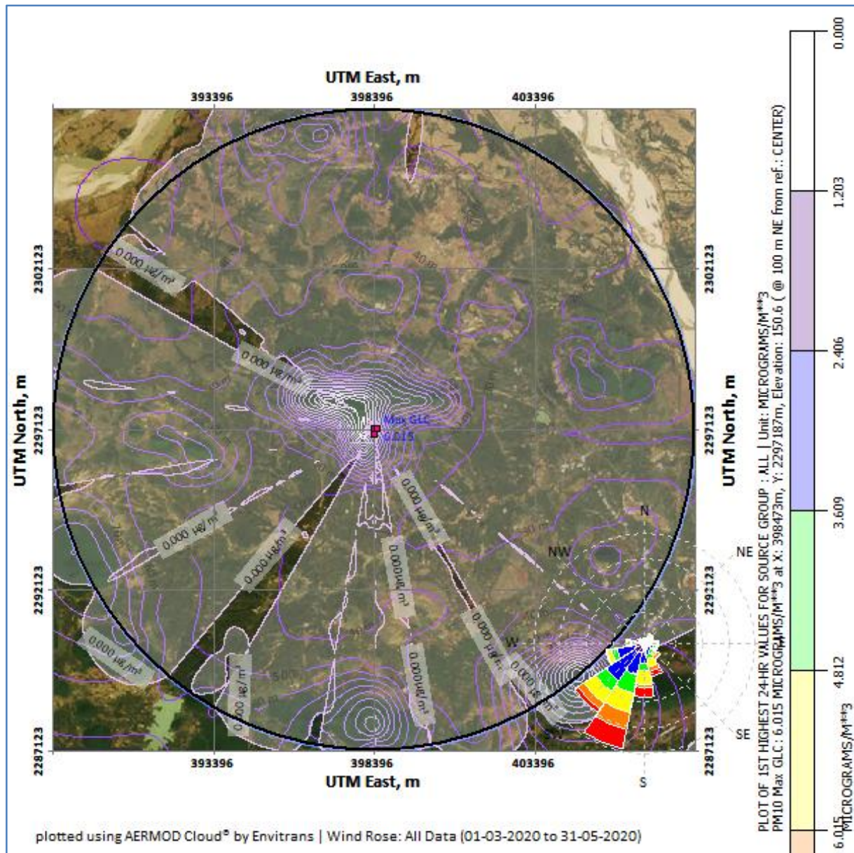
Figure 4.1 Isopleths showing incremental concentration of PM10 ( \mu\text{g}/\text{cu.m} )
