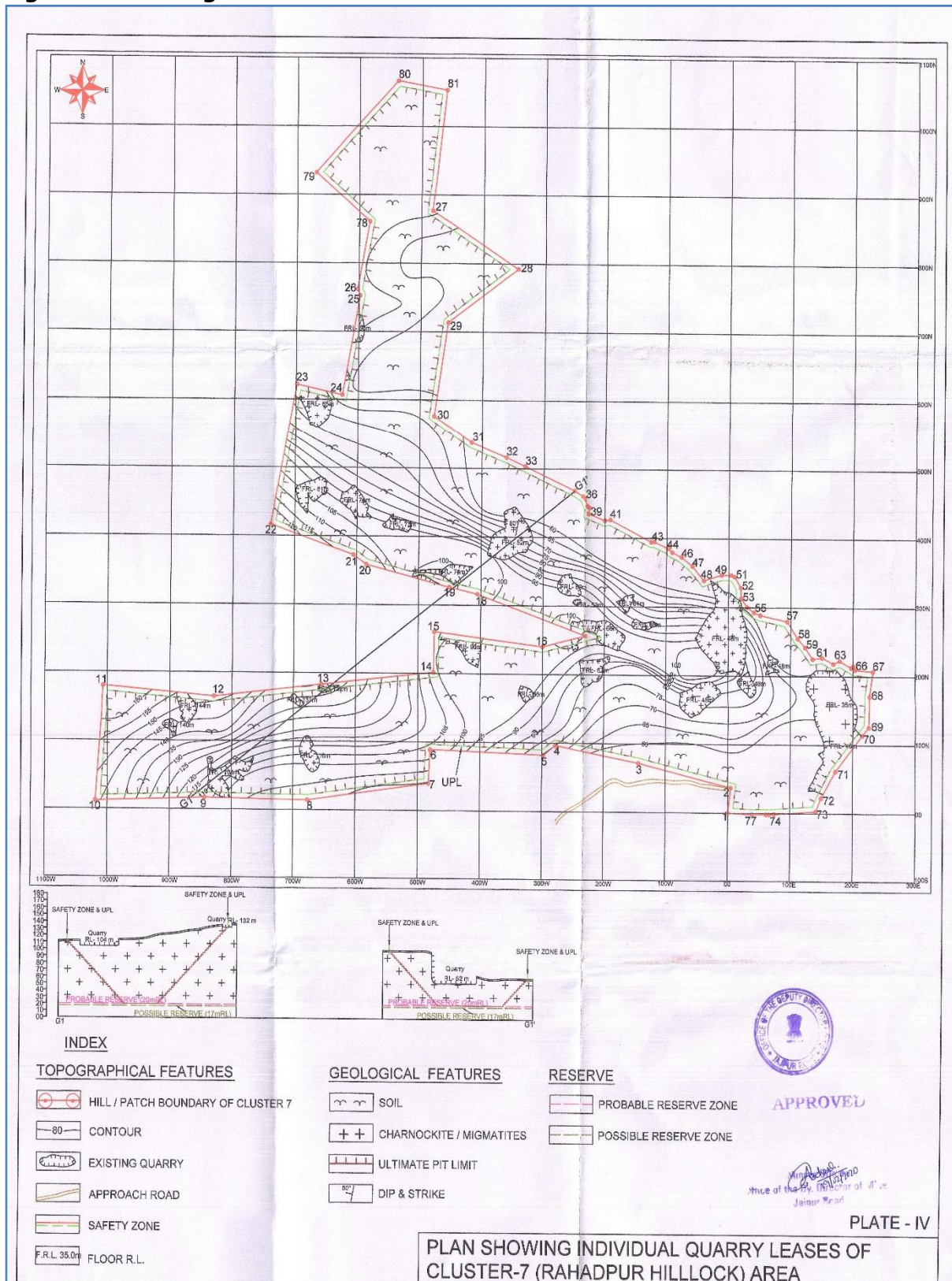
Figure 2.3: Geological Plan
